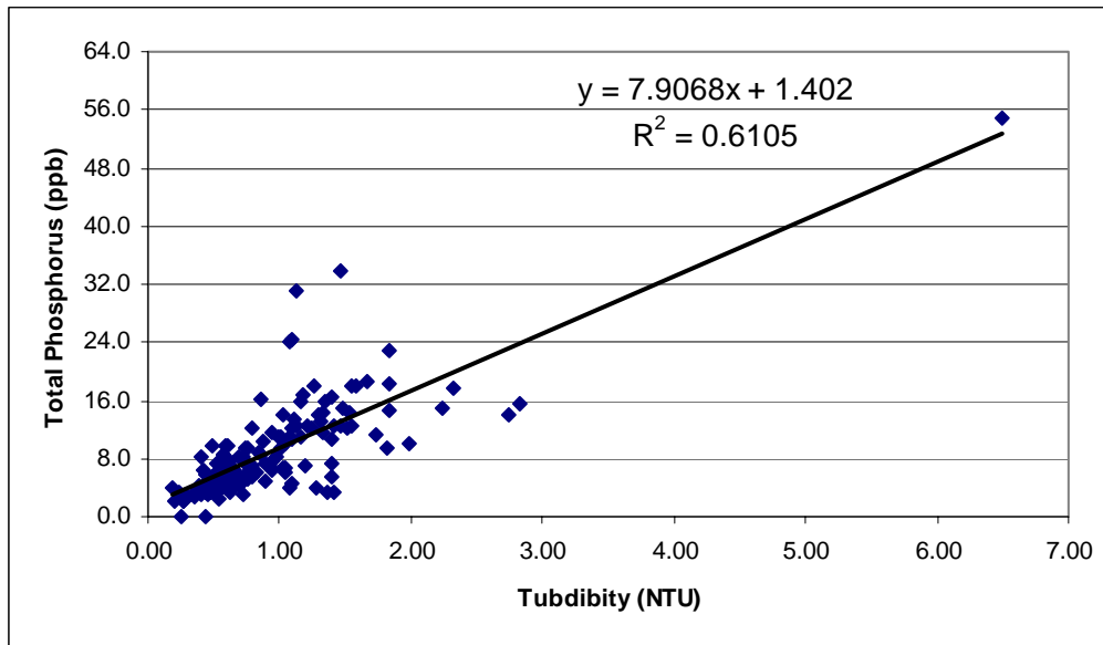
Figure 18: Total phosphorus vs. turbidity for RIVERS, 2004.
