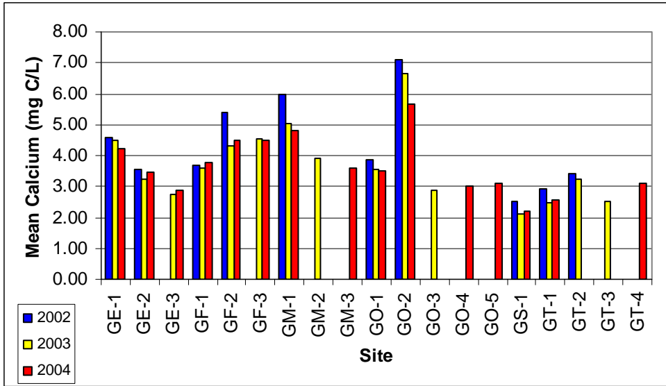
Figure 66: RIVERS site calcium comparison for 2002, 2003, and 2004.
