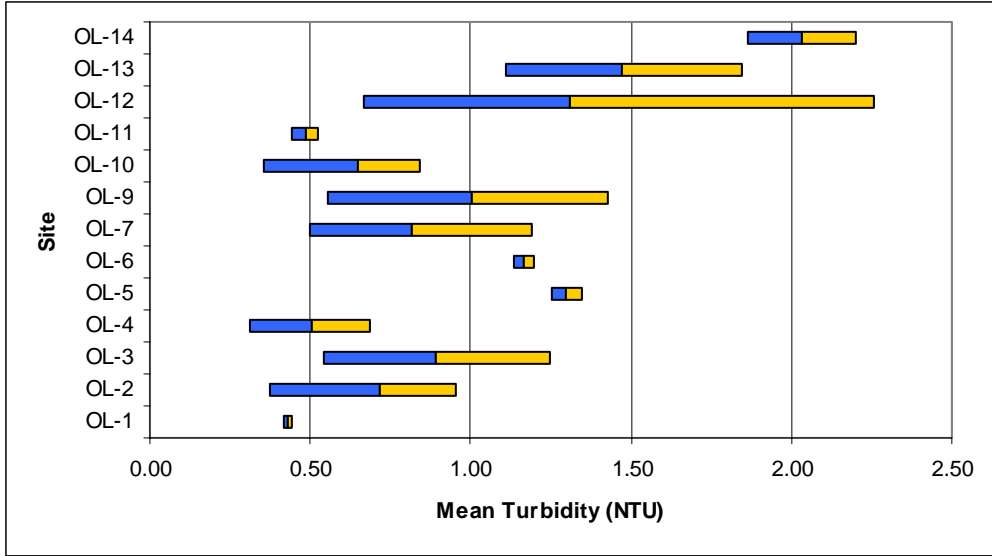
Figure 22: OLT inter site turbidity comparison. Bars show range of turbidity. Darker bars show range less than the mean. Lighter bars show range greater than the mean. Mean value is at point where dark and light bars meet.
